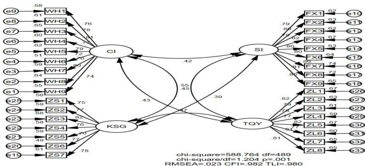
Figure 2 : Measurement Model
